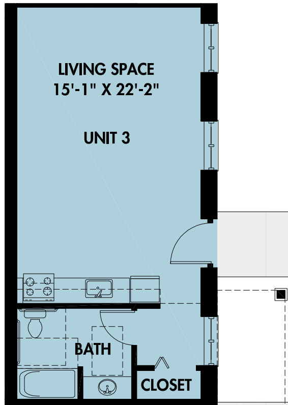
Efficiency 490 Square Feet Dimensions and Area are approximate
