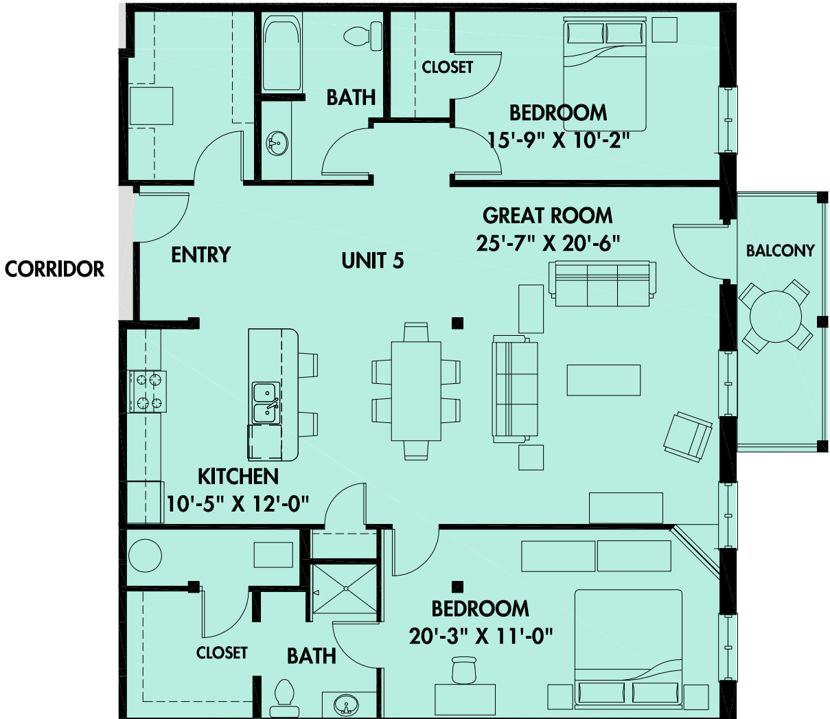
Two Bedroom 1570 Square Feet Dimensions and Area are approximate
