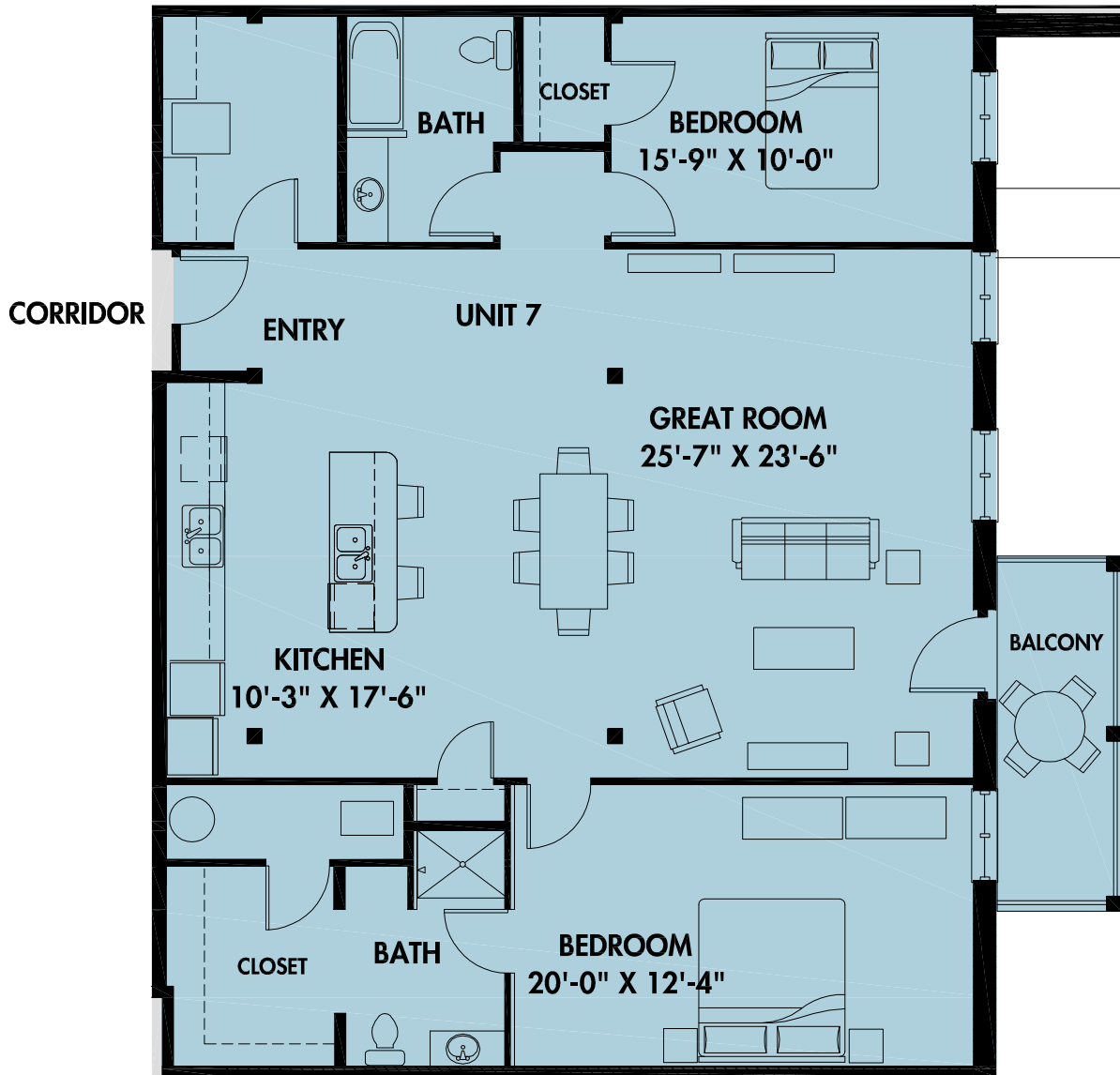
Two Bedroom 1730 Square Feet Dimensions and Area are approximate
